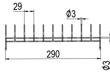
Stand Side View
