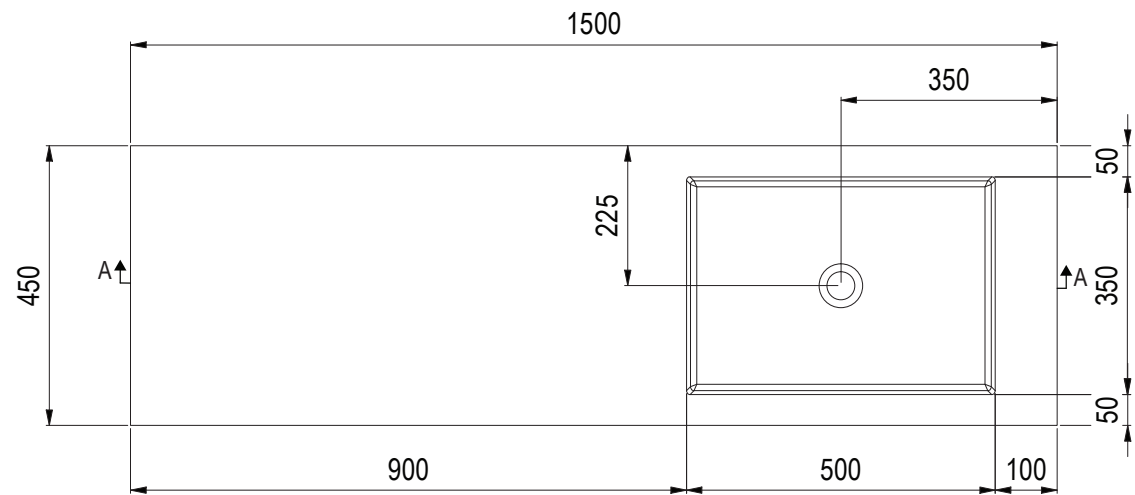
Top View
